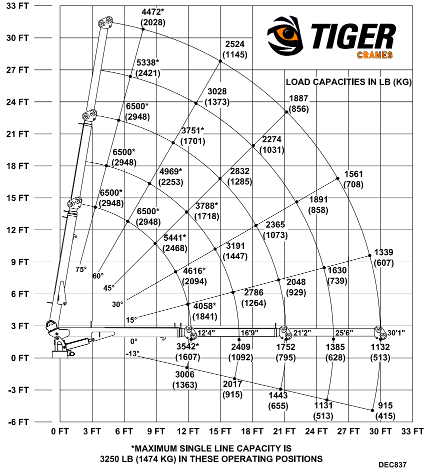
MODEL 6543 HYDRAULIC CAPACITY CHART
